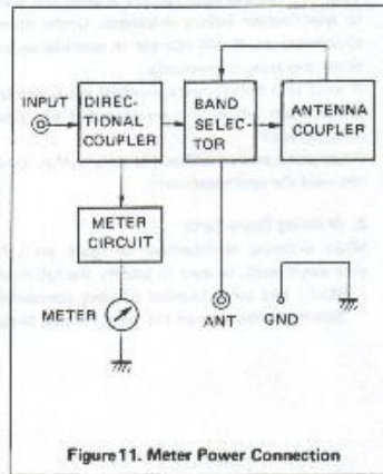
Figure 11. Meter Power Connection
