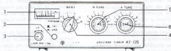
Figure 3. Front view
